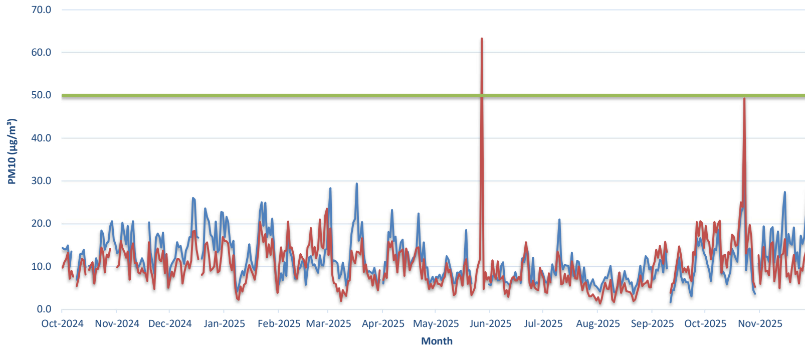
Figure 3. TEOM (PM10) Results - 12 Month Trend
