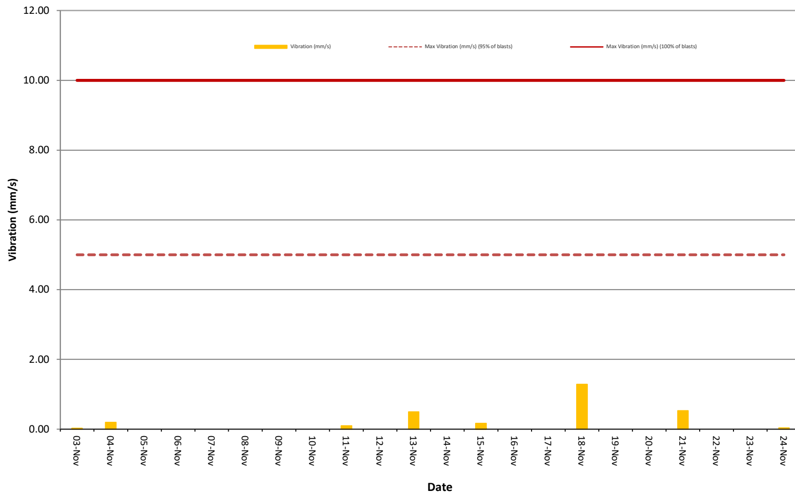
Figure 8. Vibration (mm/s) recorded during Month
