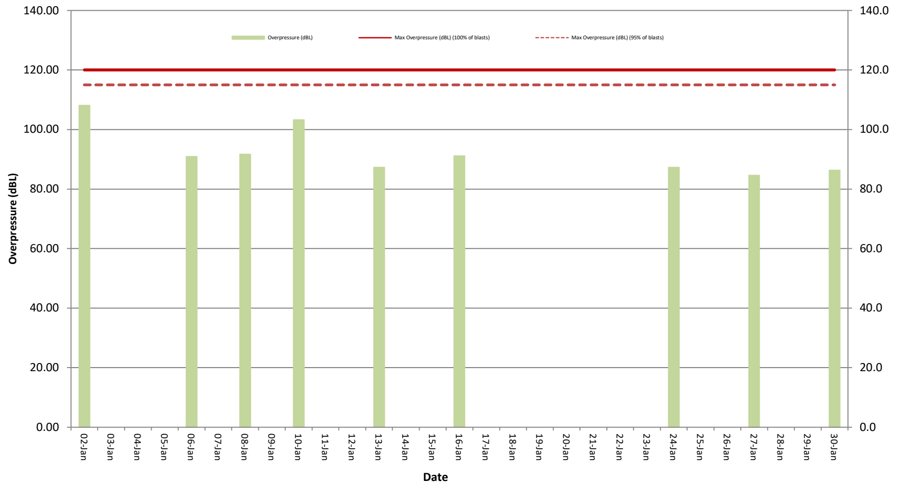
Figure 7. Overpressure (dBL) recorded during Month
