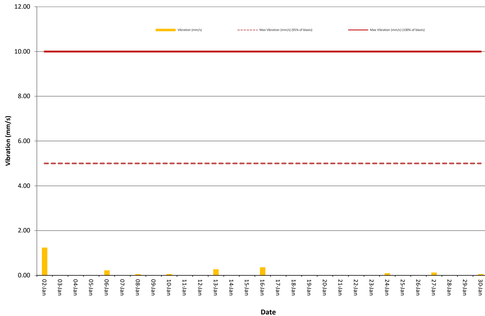
Figure 8. Vibration (mm/s) recorded during Month
