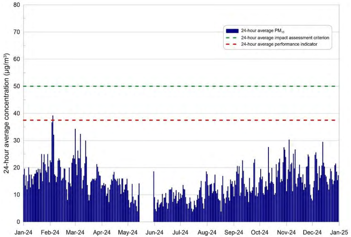
Chart 91 24-hour Average PM 10 Concentrations (measured by the TEOM)
