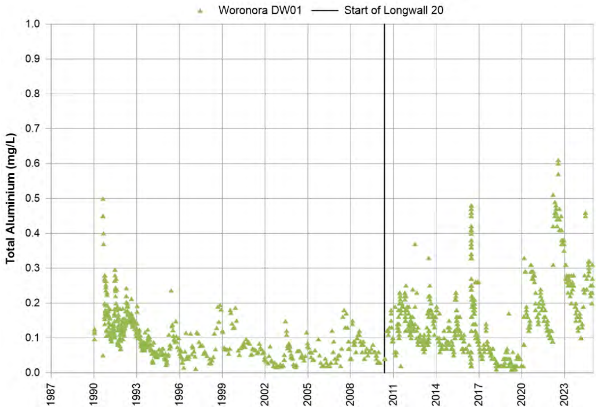
Chart 60 Total Aluminium Concentration Woronora Reservoir
