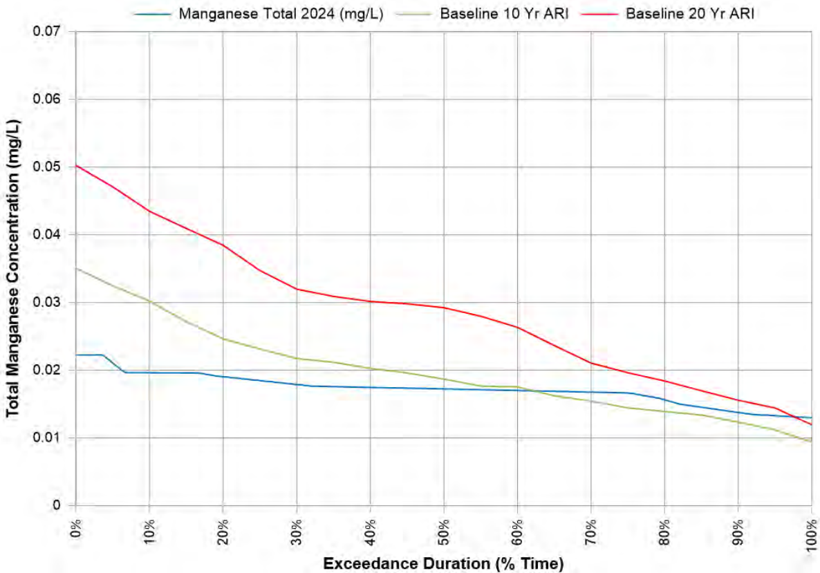
Chart 64 Total Manganese Performance Indicator Woronora Reservoir 2024
