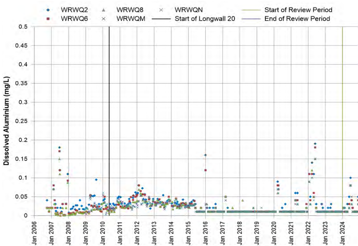
Chart 27 Dissolved Aluminium Waratah Rivulet – Upper and Middle Reach Sites
