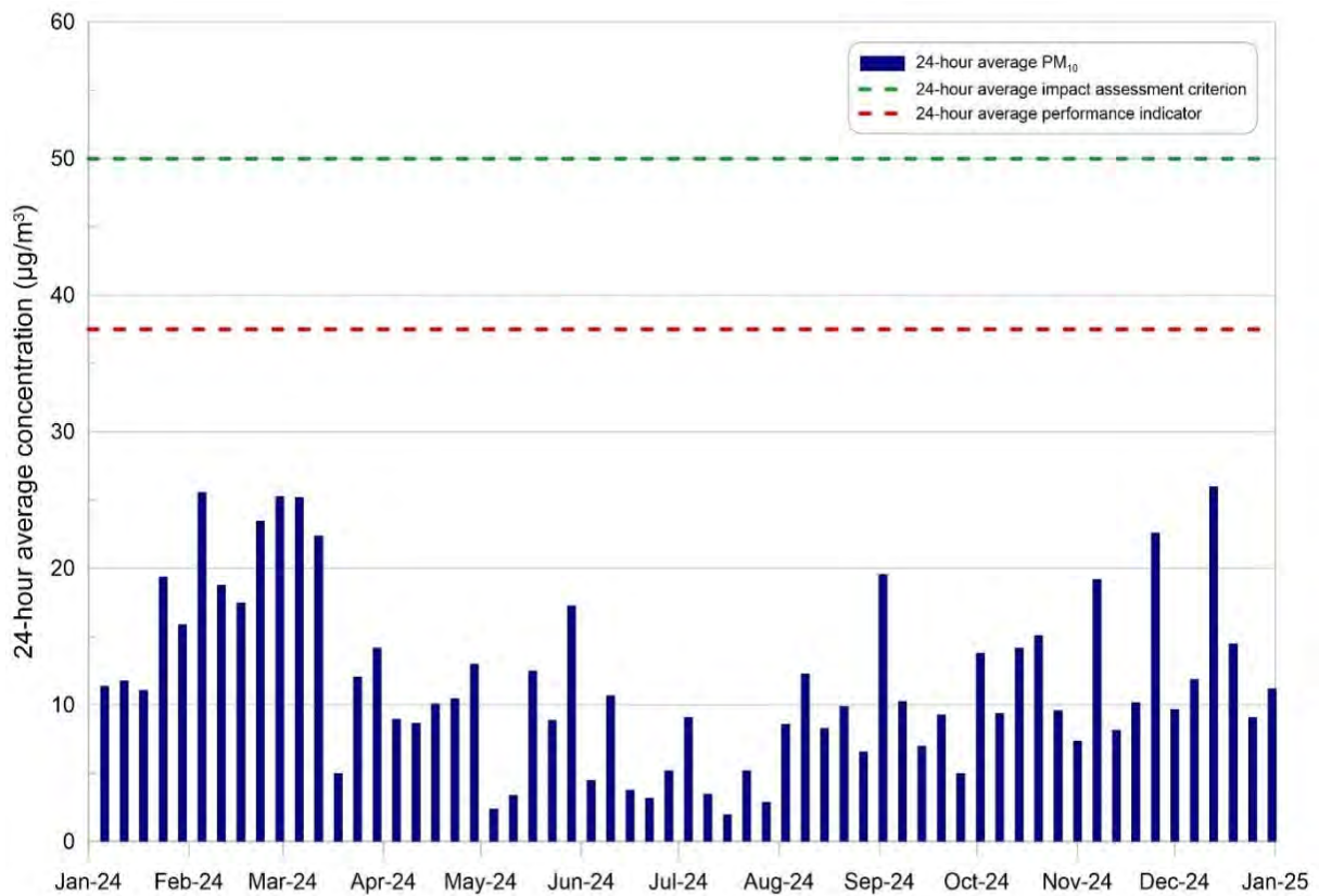
Chart 92 24-hour Average PM 10 Concentrations (measured by the HVAS)
