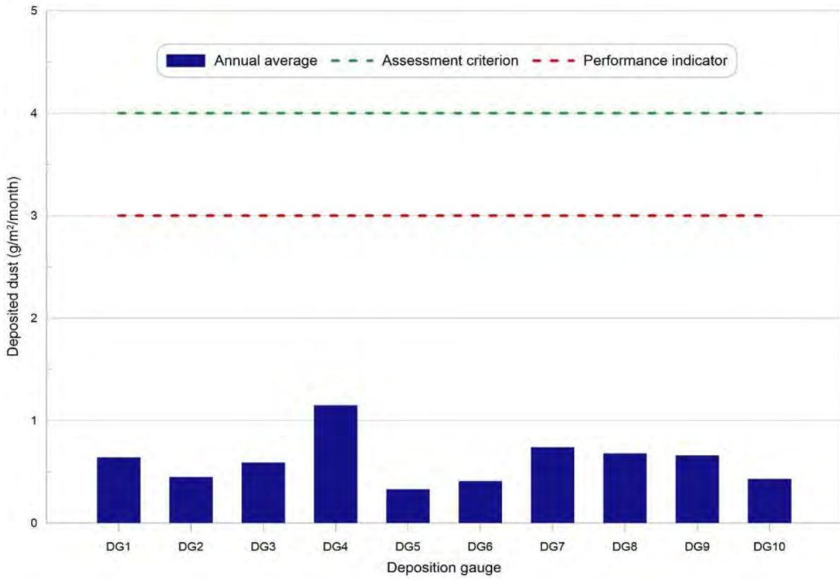
Chart 88 Annual Average Dust Deposition Rates Measured at Dust Gauges (DG1 to DG10)
