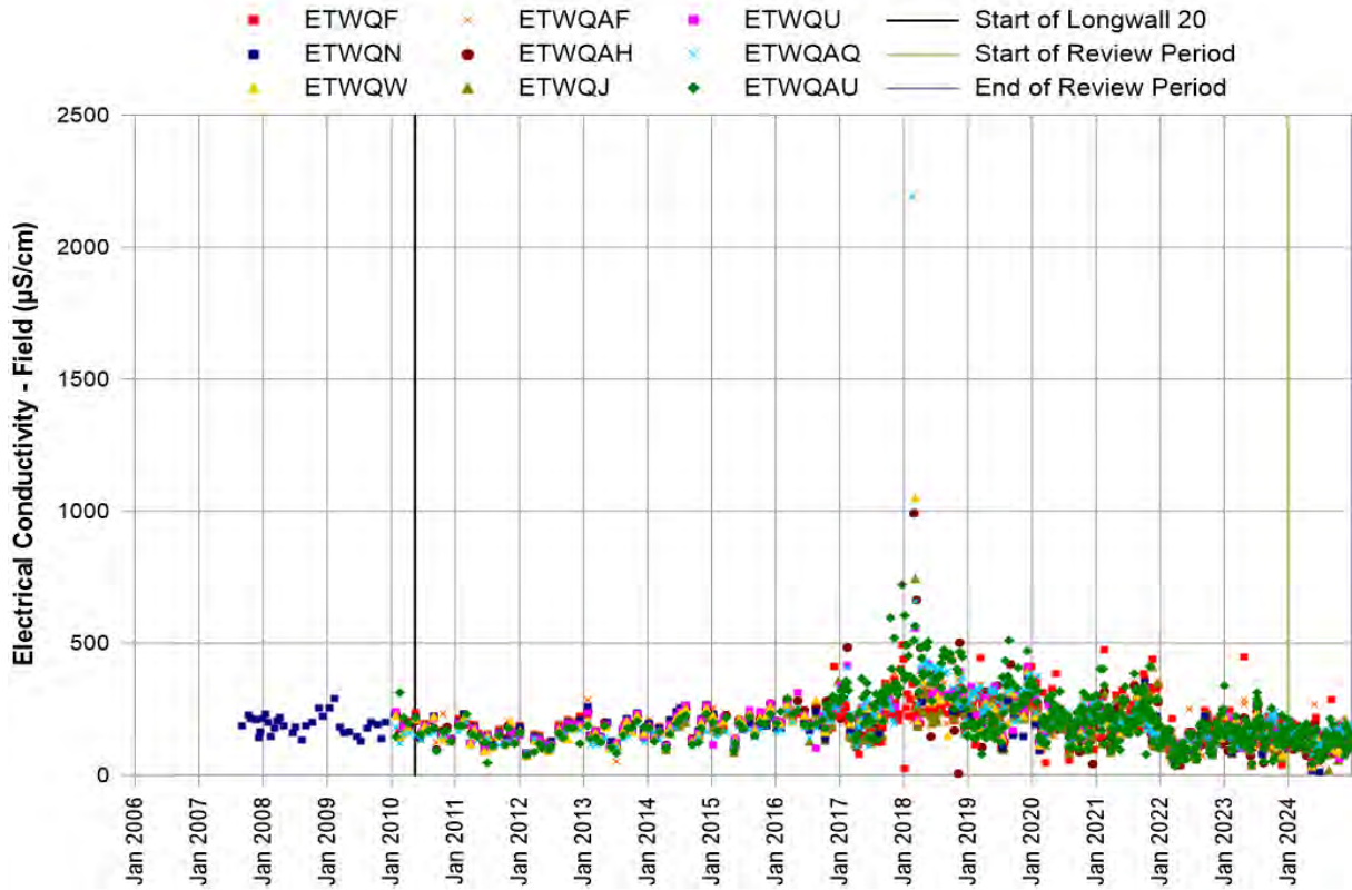
Chart 38b EC Eastern Tributary
