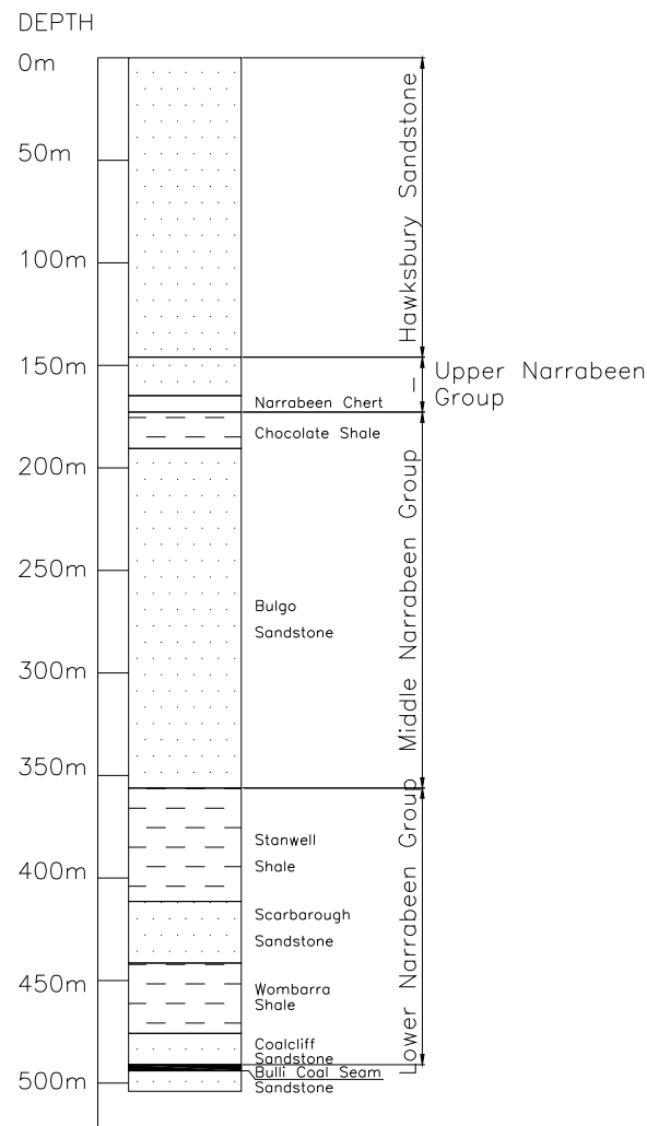
Fig. 1.3 Stratigraphic Section
