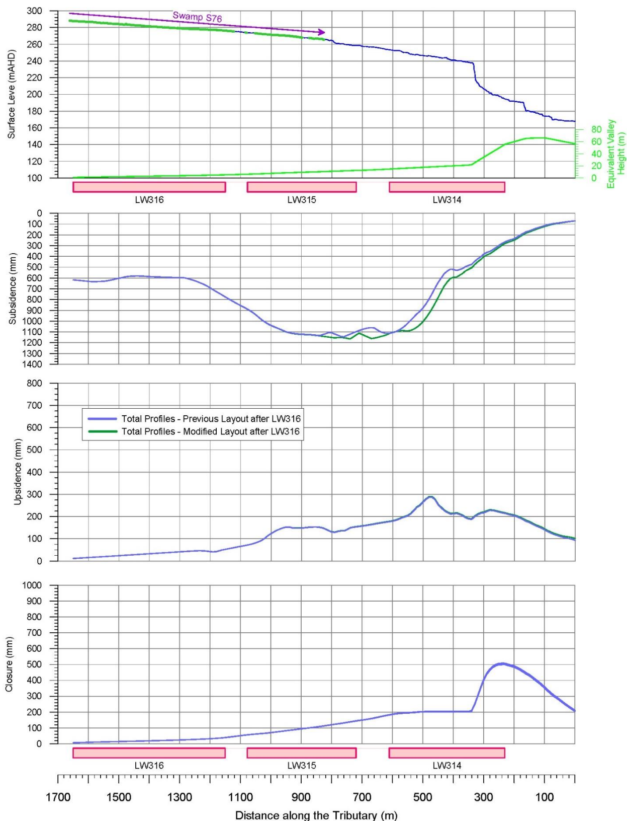
Fig. 6 Tributary S – Predicted total vertical subsident, upsidence and closure due to the Previous Layout and Modified Layout
