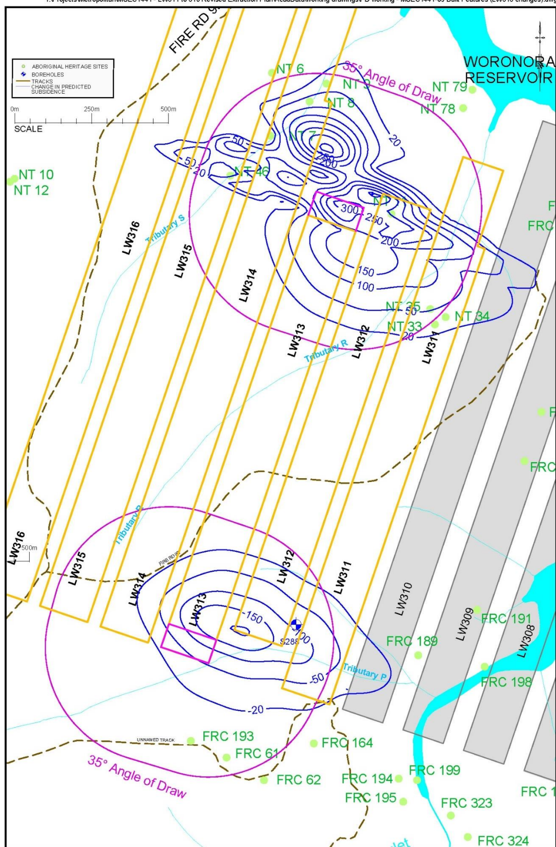
Fig. 3 Built features and Study Area for Longwall 313 changes
