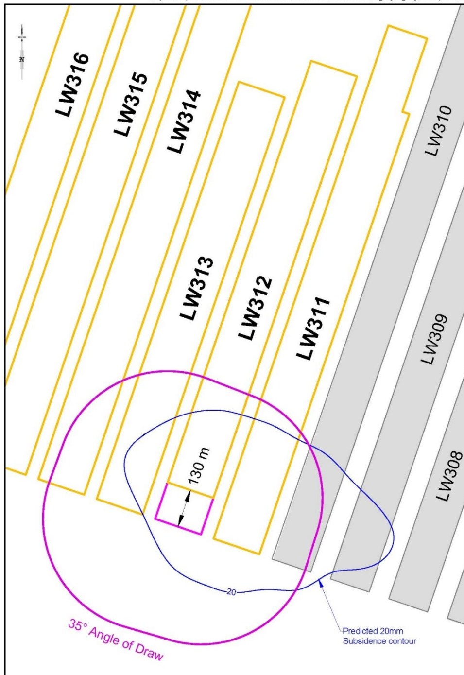
Fig. 1 Shortened Fishing end of Longwall 312 and Study Area
