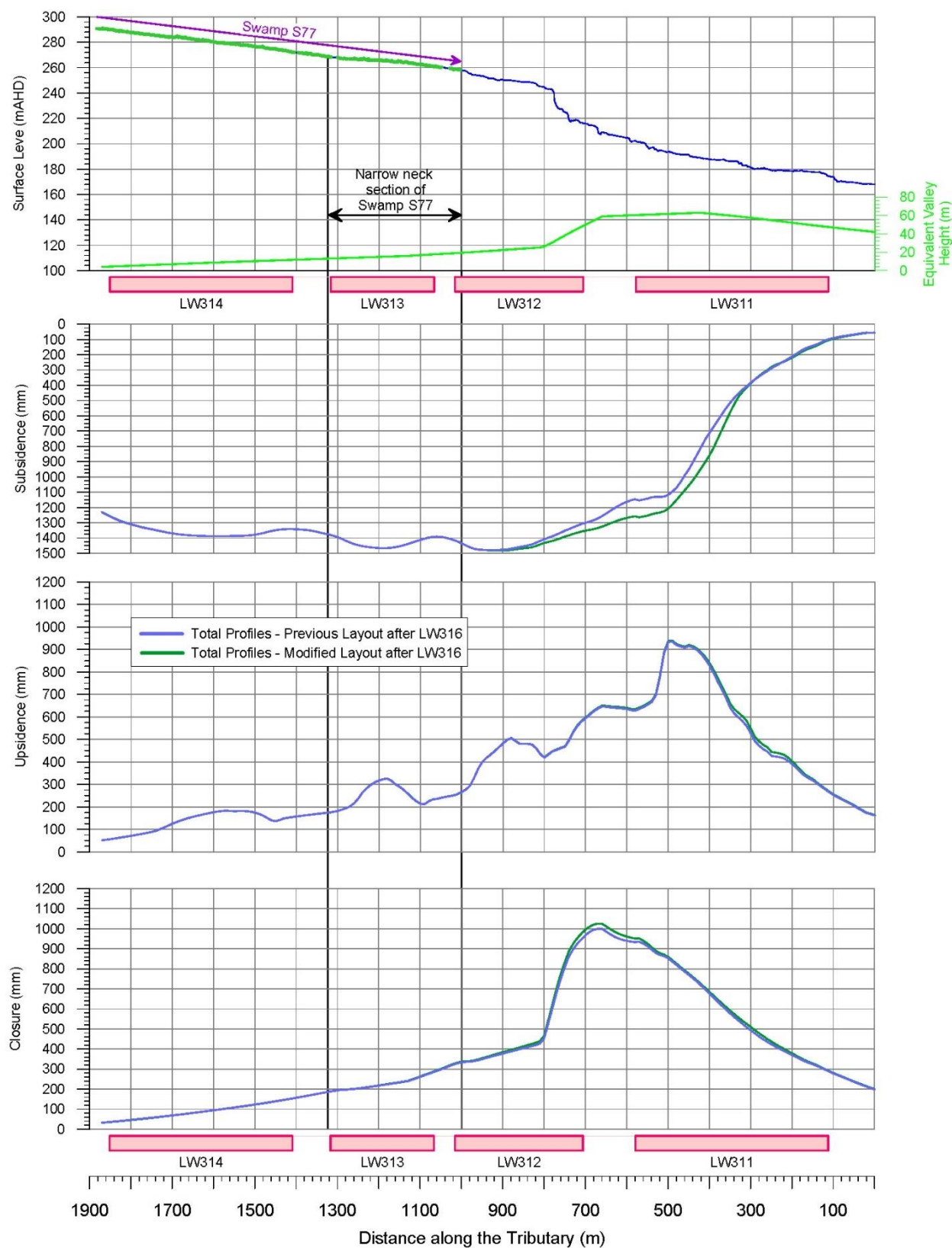
Fig. 5 Tributary R – Predicted total vertical subsident, upsidence and closure due to the Previous Layout and Modified Layout
