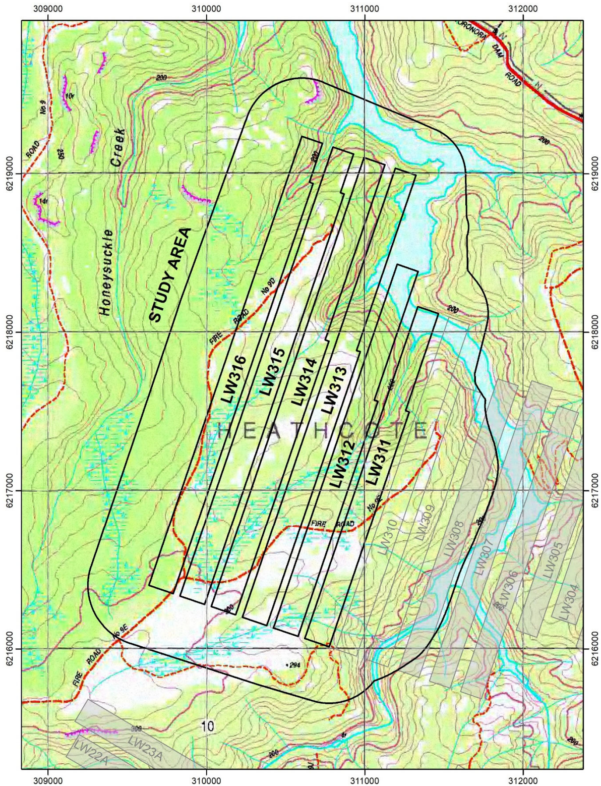
Fig. 2.1 The Proposed Longwalls 311 to 316 Overlaid on CMA Map No. Appin 9029-1S
