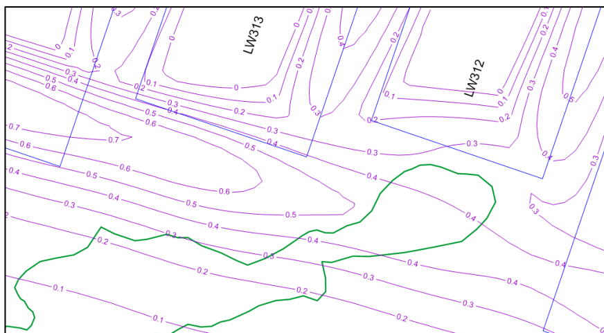
Fig. 7 Contours of predicted conventional tensile strain near Swamp S92
