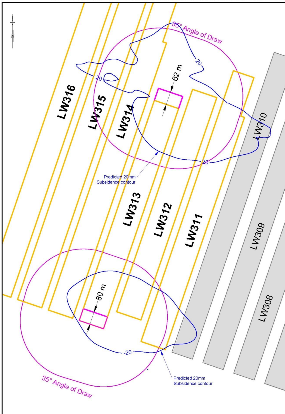
Fig. 1 Longwall 313 and Study Area
