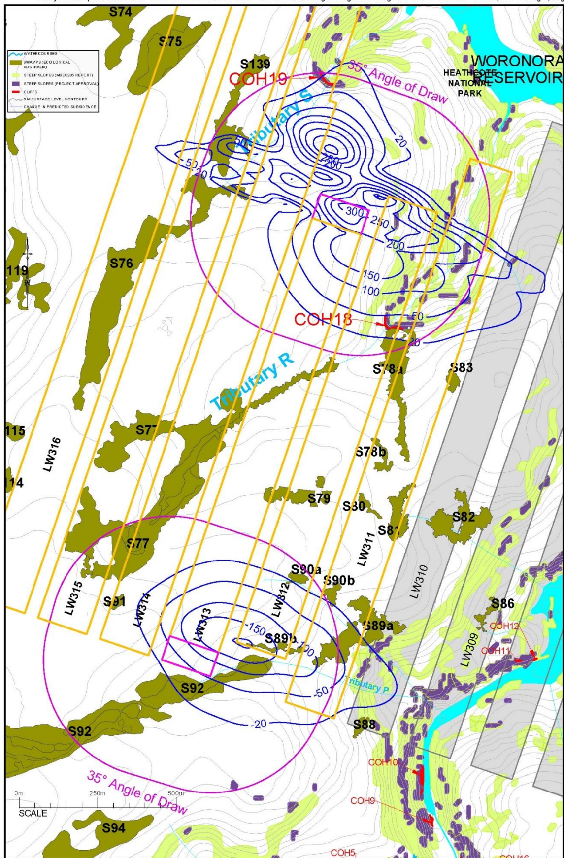
Fig. 2 Natural features and Study Area for Longwall 313 changes
