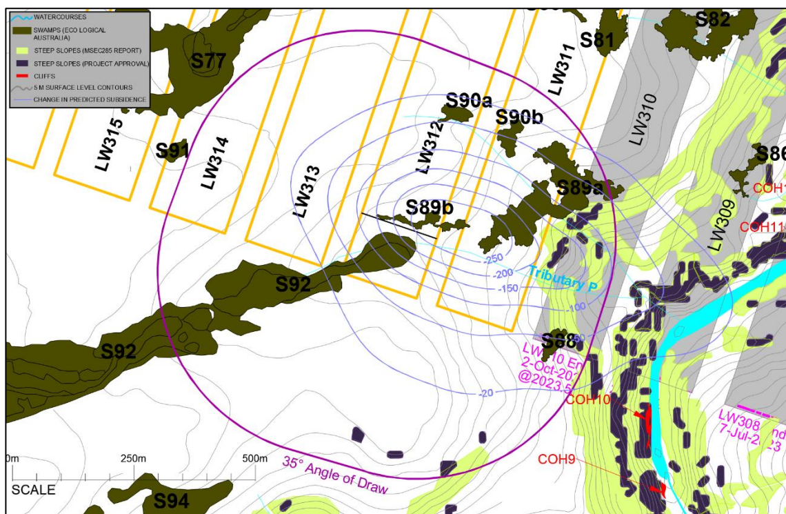
Fig. 2 Natural features and Study Area for Longwall 312 shortening
